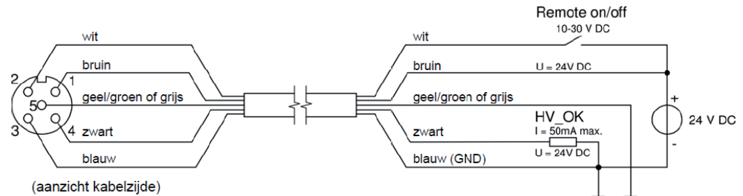
Bedrading, Performax Easy
